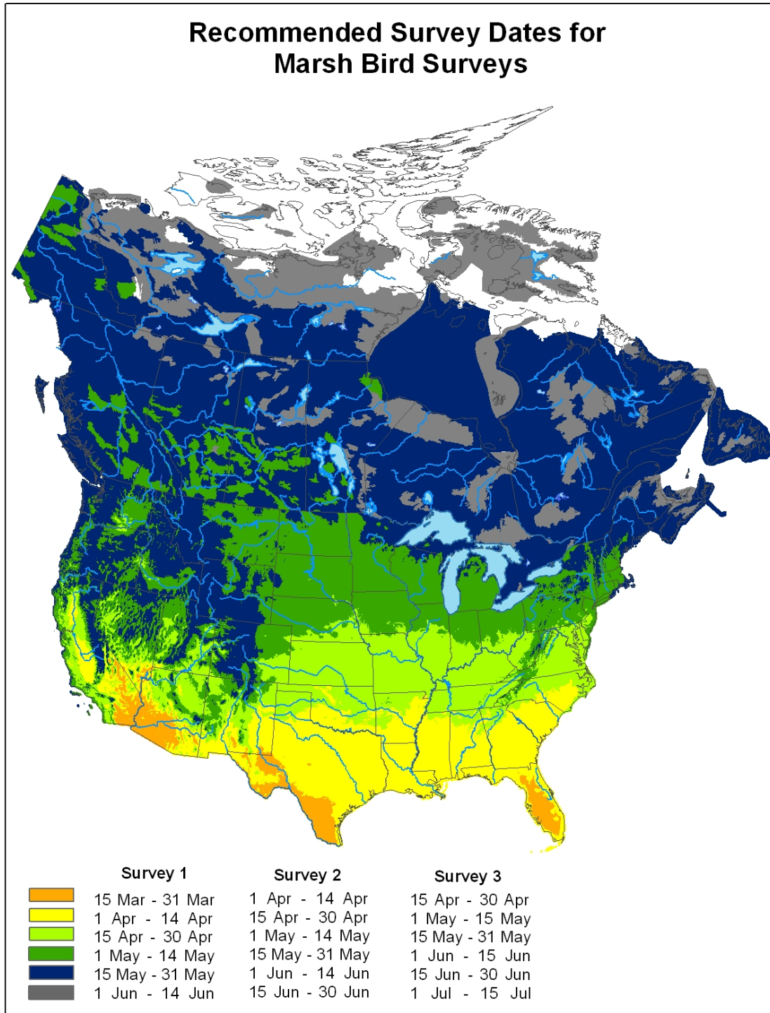
Figure B.1 Recommended dates of 3 annual survey windows for different areas in North America. The isoclines are based on average maximum temperatures in May, from PRISM at Oregon State University (for the U.S.) and Environment Canada (for Canada).
